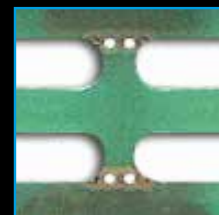
2mm Stamp
